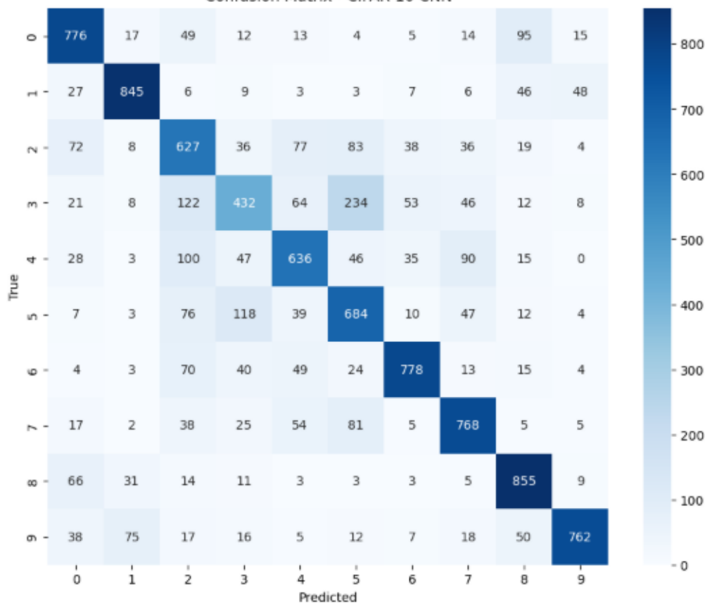
Confusion Matrix - CIFAR-10 CNN
